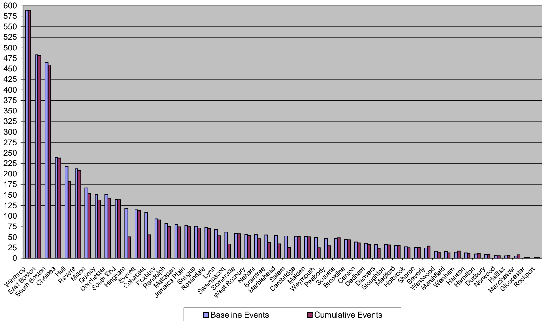
Graph 3 - Phase 1 BLANS Alternatives Community Average Baseline and Cumulative Average Daily Events Above 65 SEL (Level Approximates Normal Conversation at 8 Feet)
